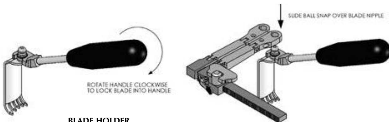
BLADE HOLDER
